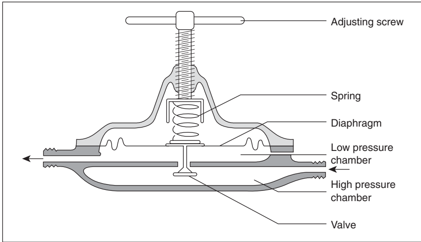
Figure 7.1 A pressure-reducing valve.
