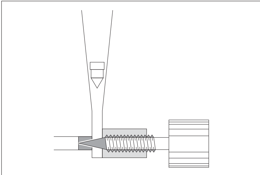
Figure 7.2 Flow meter needle valve and rotameter.
